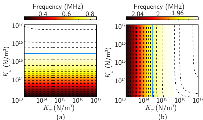
FIG. 9. Theoretical evolution of the frequency of the modes S_1S_2 (a) and A(S_1S_2) (b) as a function of both interfacial stiffnesses in the range [10^{13}; 10^{17}] N/m 3 . Dashed lines correspond to isofrequency curves. Solid lines correspond to f_{S_1S_2} = 0.836 MHz (a) and f_{A(S_1S_2)} = 2.055 MHz (b).
