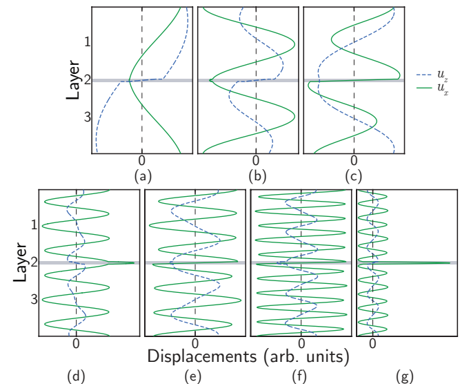
FIG. 3. Theoretical normal (dashed line) and in-plane (solid line) displacements, in a Duralumin/epoxy/Duralumin structure with K_L = K_T = 5 \times 10^{14} \text{ N/m}^3 and h = 50 \text{ }\mu\text{m} , for ZGV Lamb modes (a) S_1S_2 (0.744 MHz), (b) S(S_1S_2) (2.022 MHz), (c) A(S_1S_2) (2.032 MHz), (d) S(S_3S_6)^* (6.173 MHz), (e) A(S_3S_6)^* (6.222 MHz), (f) A(S_5S_{10})^* (10.403 MHz) and (g) S(S_5S_{10})^* (10.685 MHz).
