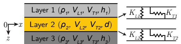
FIG. 1. Geometry of the tri-layer model.
