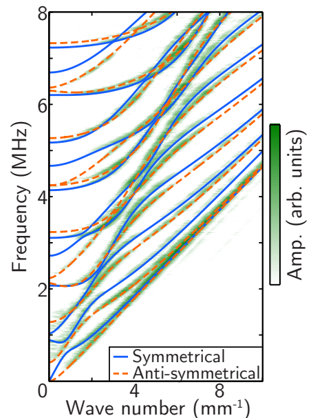
FIG. 10. Experimental (map) and theoretical (solid and dashed lines) dispersion curves obtained with the measured stiffnesses K_L = 2.52 \times 10^{15} N/m 3 and K_T = 2.83 \times 10^{14} N/m 3 .
