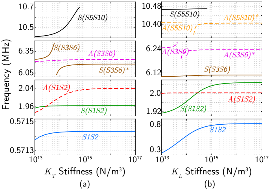
FIG. 6. Theoretical ZGV modes of the tri-layer structure with d = 50 \mu\text{m} as a function of (a) the stiffness K_T evolving from 10^{13} \text{ N/m}^3 to 10^{17} \text{ N/m}^3 with K_L = 10^{14} \text{ N/m}^3 and of (b) the stiffness K_L evolving from 10^{13} \text{ N/m}^3 to 10^{17} \text{ N/m}^3 with K_T = 10^{14} \text{ N/m}^3 . Symmetrical modes (solid line) and anti-symmetrical modes (dashed line).
