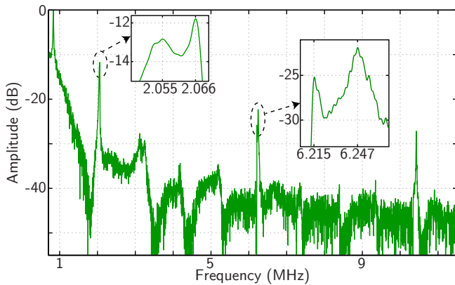
FIG. 8. Experimental signal obtained by transmission in the Duralumin/epoxy/Duralumin tri-layer structure.
