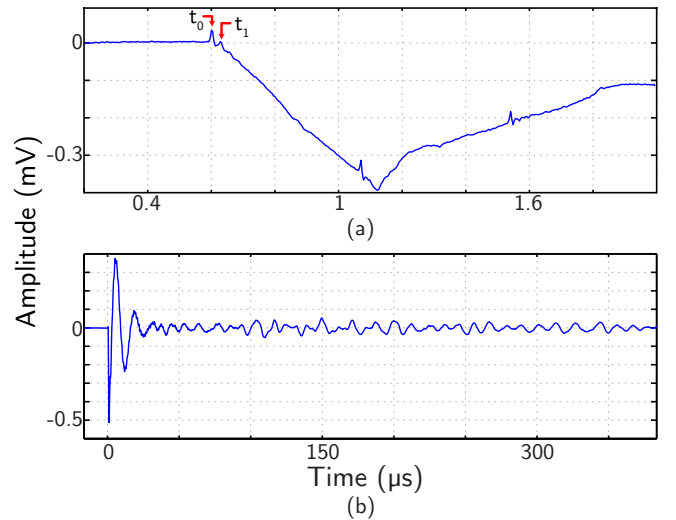
FIG. 7. Typical signal measured by transmission in the Duralumin/epoxy/Duralumin structure: (a) at short arrival time with a \sim 100 μm beam diameter to observe first reflections in the intermediate layer, (b) with a beam diameter of \sim 3 mm to enhance ZGV mode resonances.
