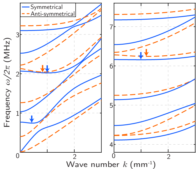
FIG. 2. Theoretical dispersion curves for a Duralumin/epoxy/Duralumin sample, with K_L = K_T = 5 \times 10^{14} \text{ N/m}^3 and h = 50 \text{ }\mu\text{m} . Arrows indicate ZGV Lamb mode frequencies.
